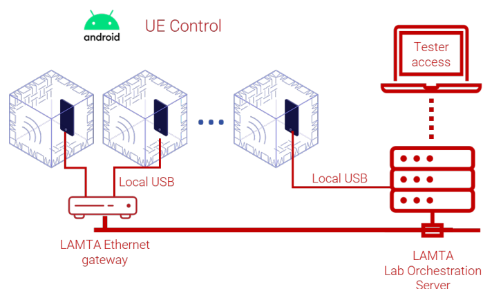
Fig1. Users can control local and remote UE simultaneously from the LAMTA GUI. UE resources can also be assigned to specific users to avoid testing interruptions.
